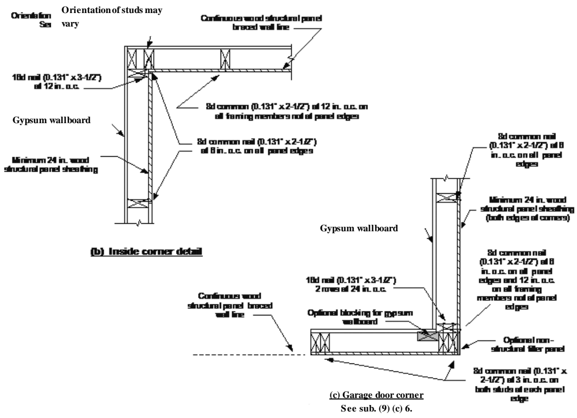
FIGURE 21.25-G TYPICAL EXTERIOR CORNER FRAMING FOR CONTINUOUS STRUCTURAL PANEL SHEATHING SHOWING REQUIRED STUD-TO-STUD NAILING
